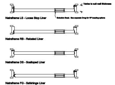
Standard Frame Details
